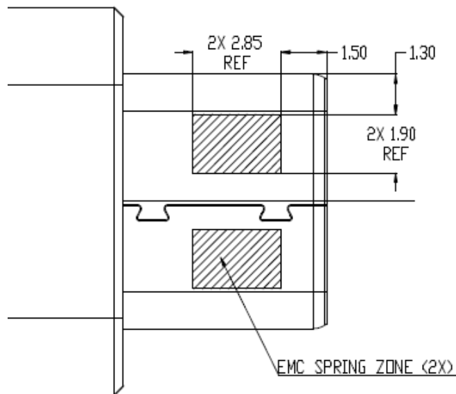
Figure 3-2 Reference Design USB Type-C Plug External EMC Spring Contact Zones 插头外部EMC弹簧触点区域
