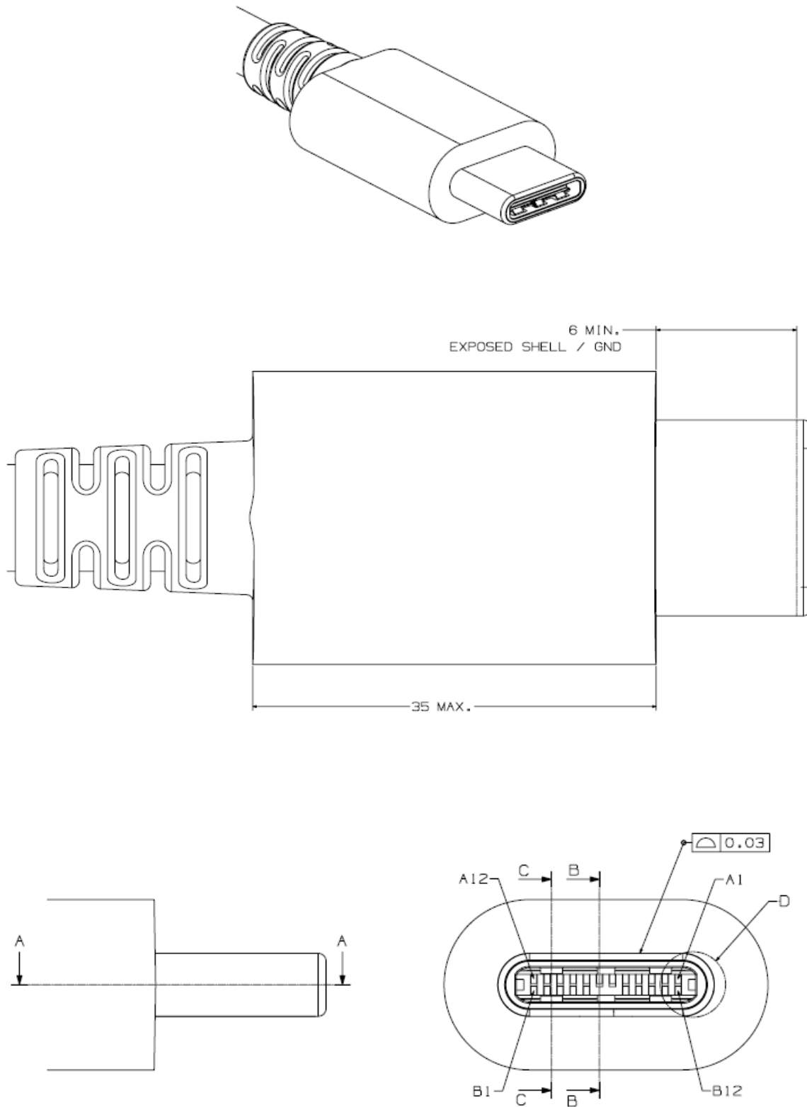
Figure 3-3 USB Full-Featured Type-C Plug Interface Dimensions 插头接口尺寸
