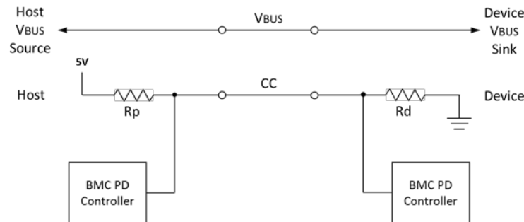
Figure 4-32 USB PD over CC Pins
