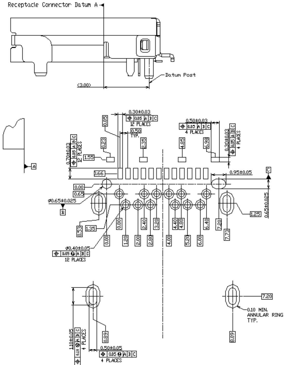
Figure 3-6 Reference Footprint for a USB Type-C Hybrid Right-Angle Receptacle (Informative) 混合直角插座
