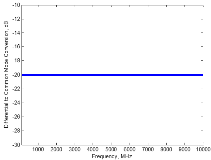
Figure 3-40 Differential-to-Common-Mode Conversion Requirement
