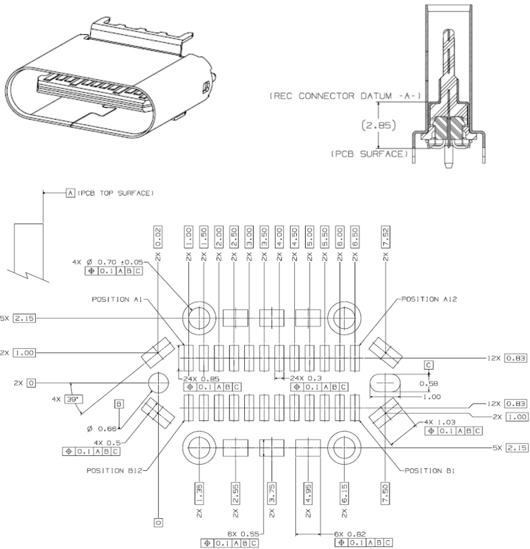
Figure 3-4 Reference Footprint for a USB Type-C Vertical Mount Receptacle (Informative) 垂直安装插座
