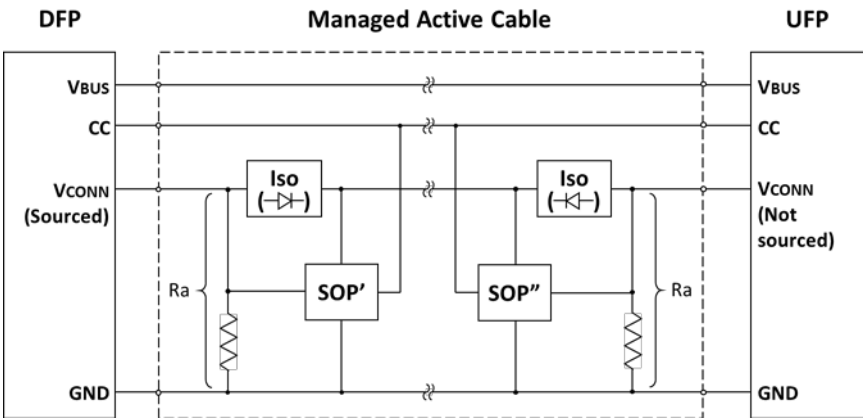
Figure 5-7 Managed Active Cable
