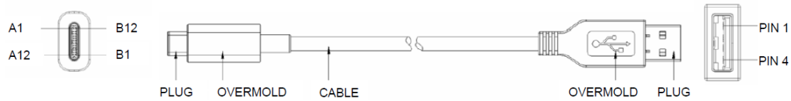
Figure 3-23 USB Type-C to USB 2.0 Standard-A Cable Assembly
