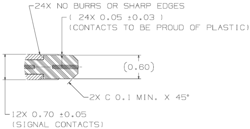
DETAIL D
